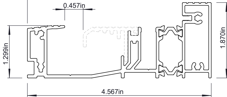
Sill Thermally broken aluminum
